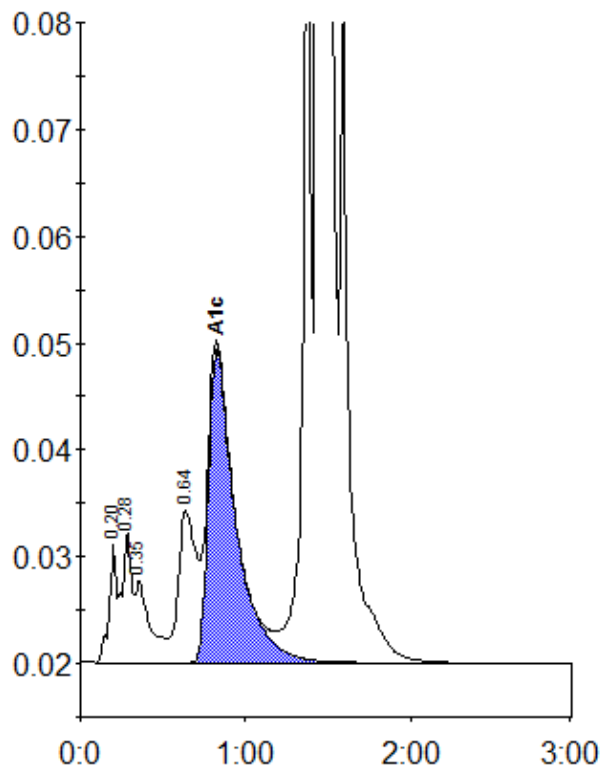
Peak table - ID: 10342889
